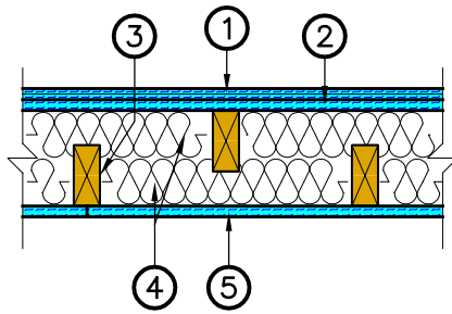
TEST #1112 HORIZONTAL WALL SECTION SCALE: 1"=1'-0"
