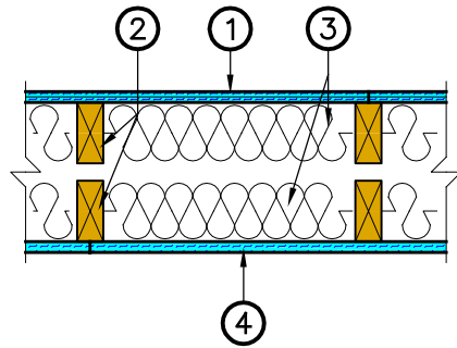
TEST #1113 HORIZONTAL WALL SECTION SCALE: 1"=1'-0"
