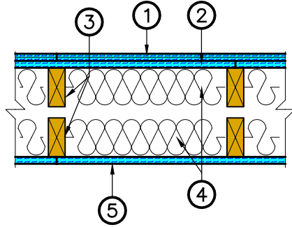
TEST #1114 HORIZONTAL WALL SECTION SCALE: 1"=1'-0"
